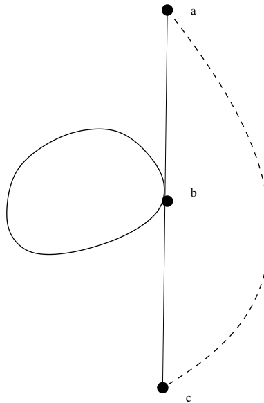
FIGURE 11. The outer caustic has the property that any tangent line to the table cuts off the segment which is divided into two equal pieces by the tangency point.
