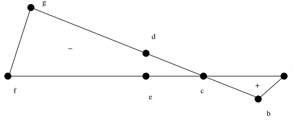
FIGURE 12. Area property of the outer caustics
