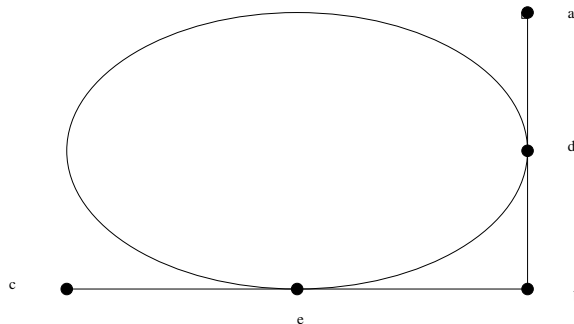
FIGURE 4. Outer billiard
