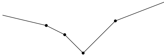
FIGURE 20. Wojtkowski wedge
